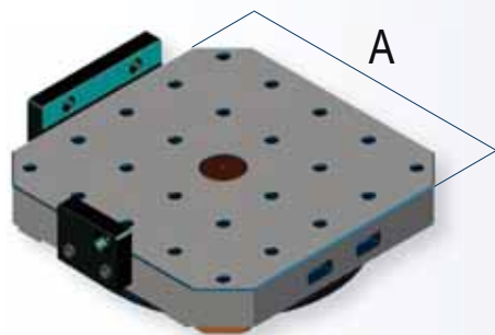
Art. 85 Pallet a reticolo con fori in tegrali M16 Grid pallet type with solid threads M16
